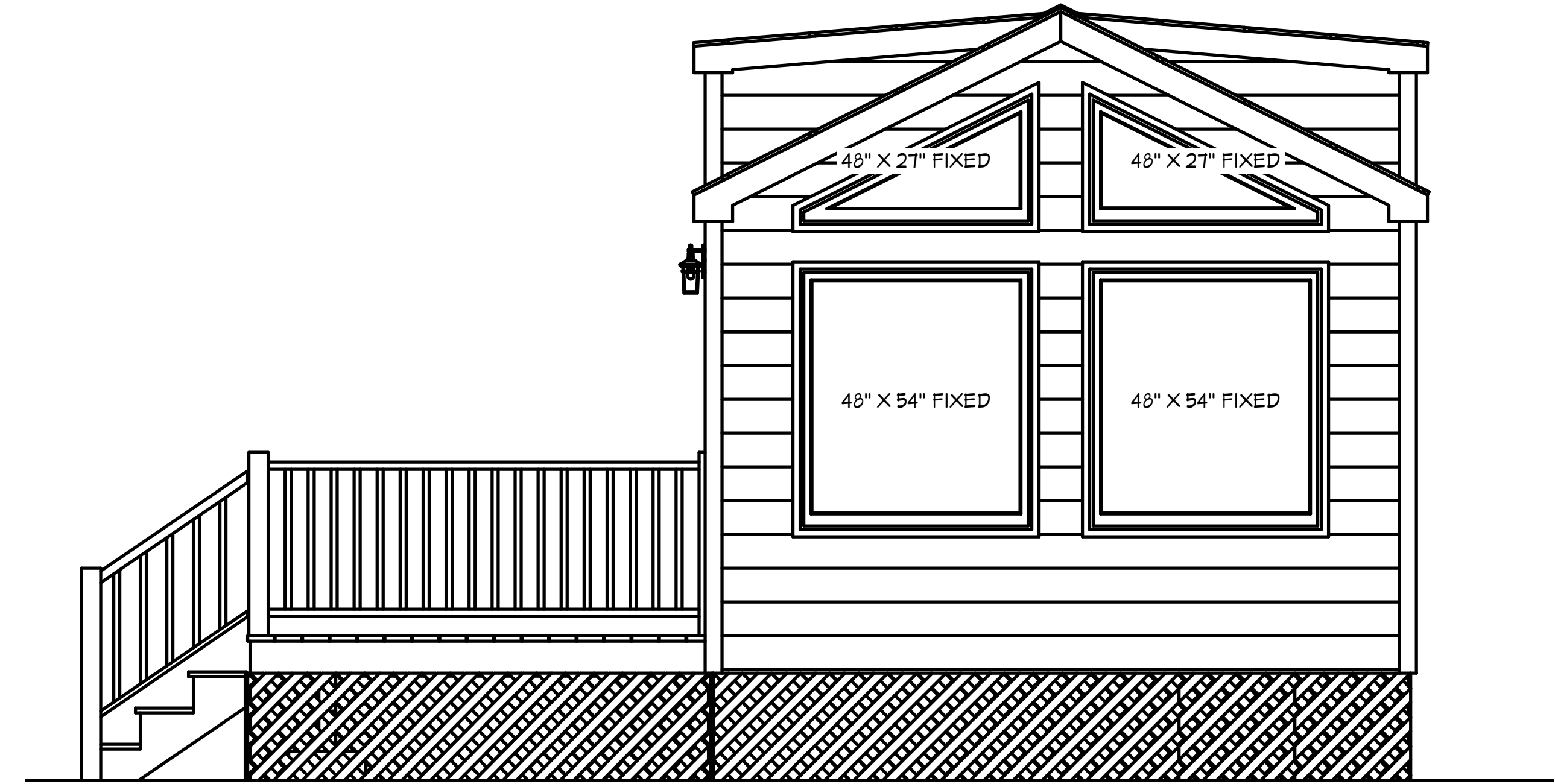
2 EXTERIOR ELEVATION RIGHT A-5 1/2 IN = 1 FT
