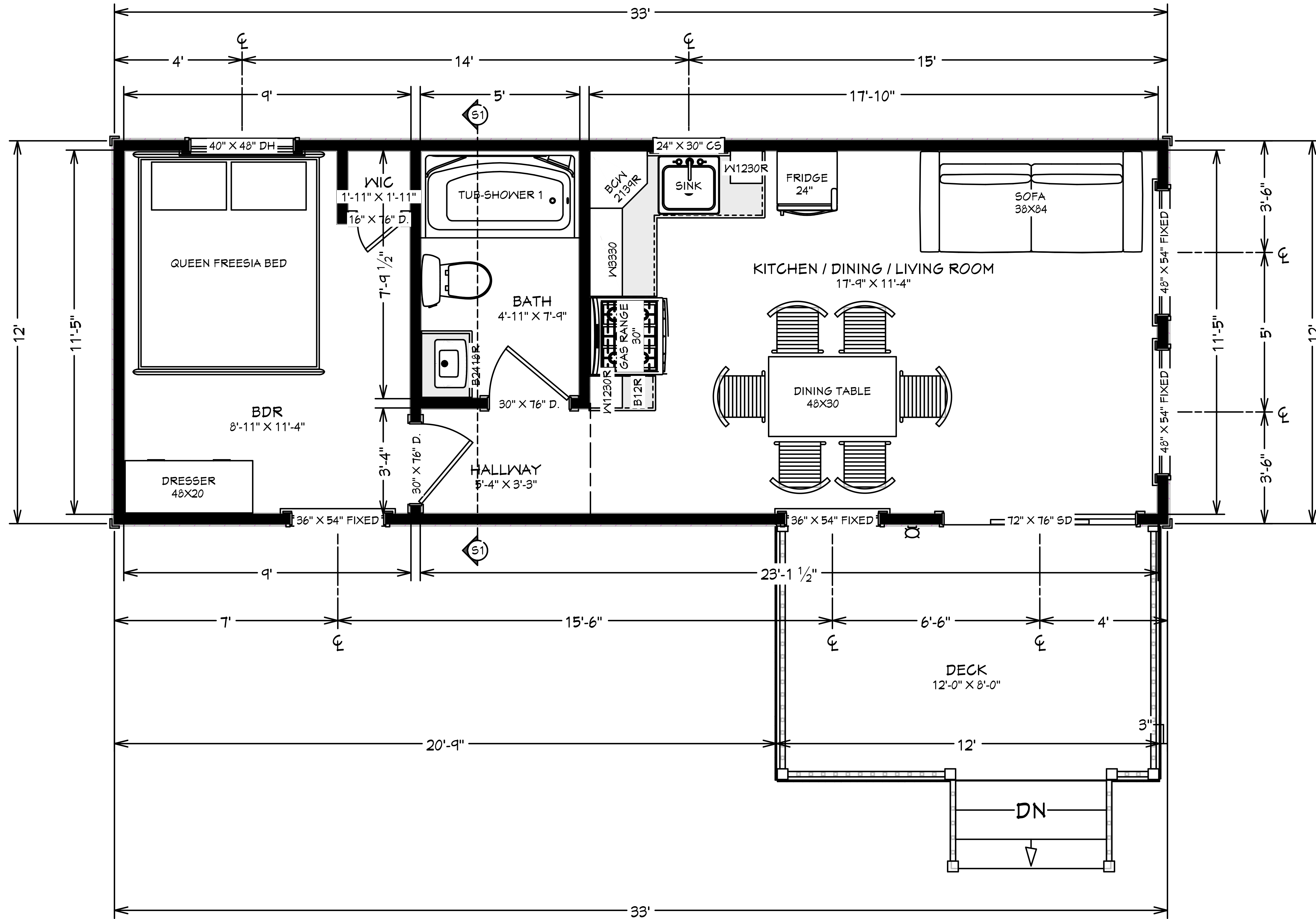
1 1ST FLOOR PLAN A-3 5/8 IN = 1 FT
