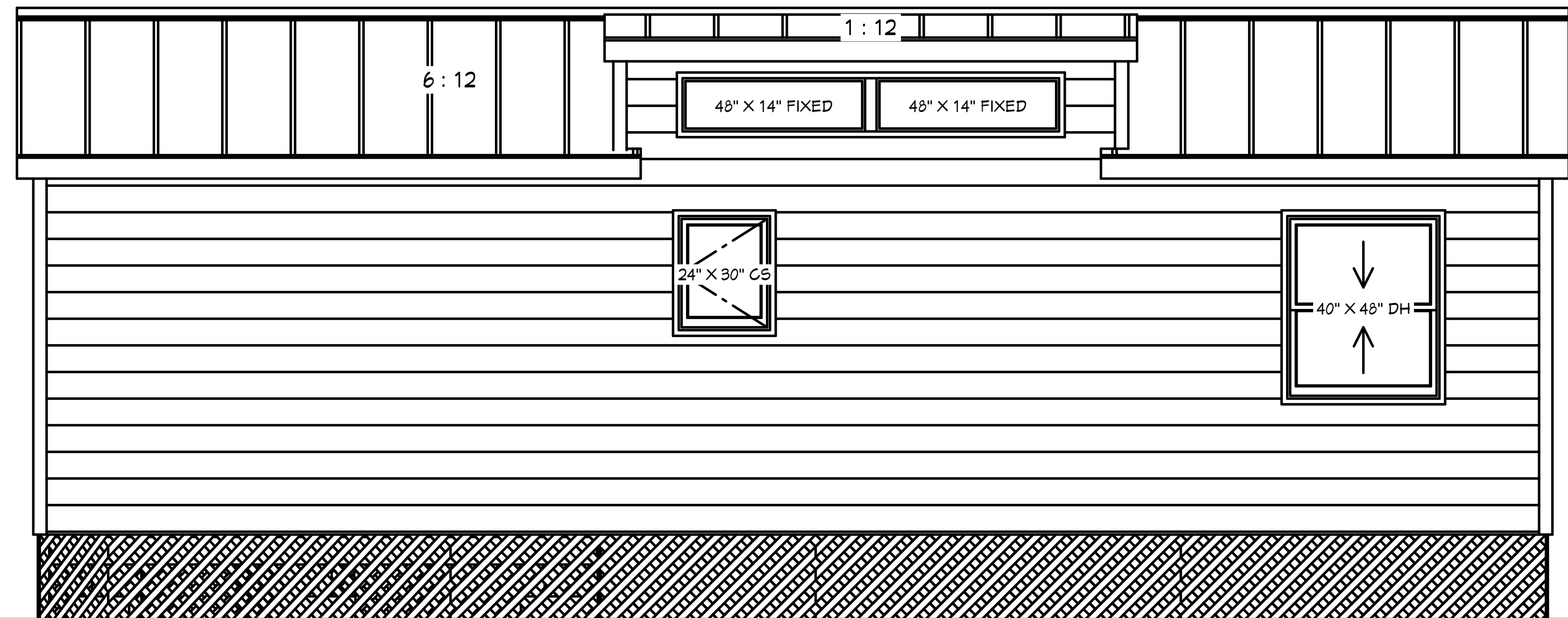
3 EXTERIOR ELEVATION BACK A-5 1/2 IN = 1 FT
