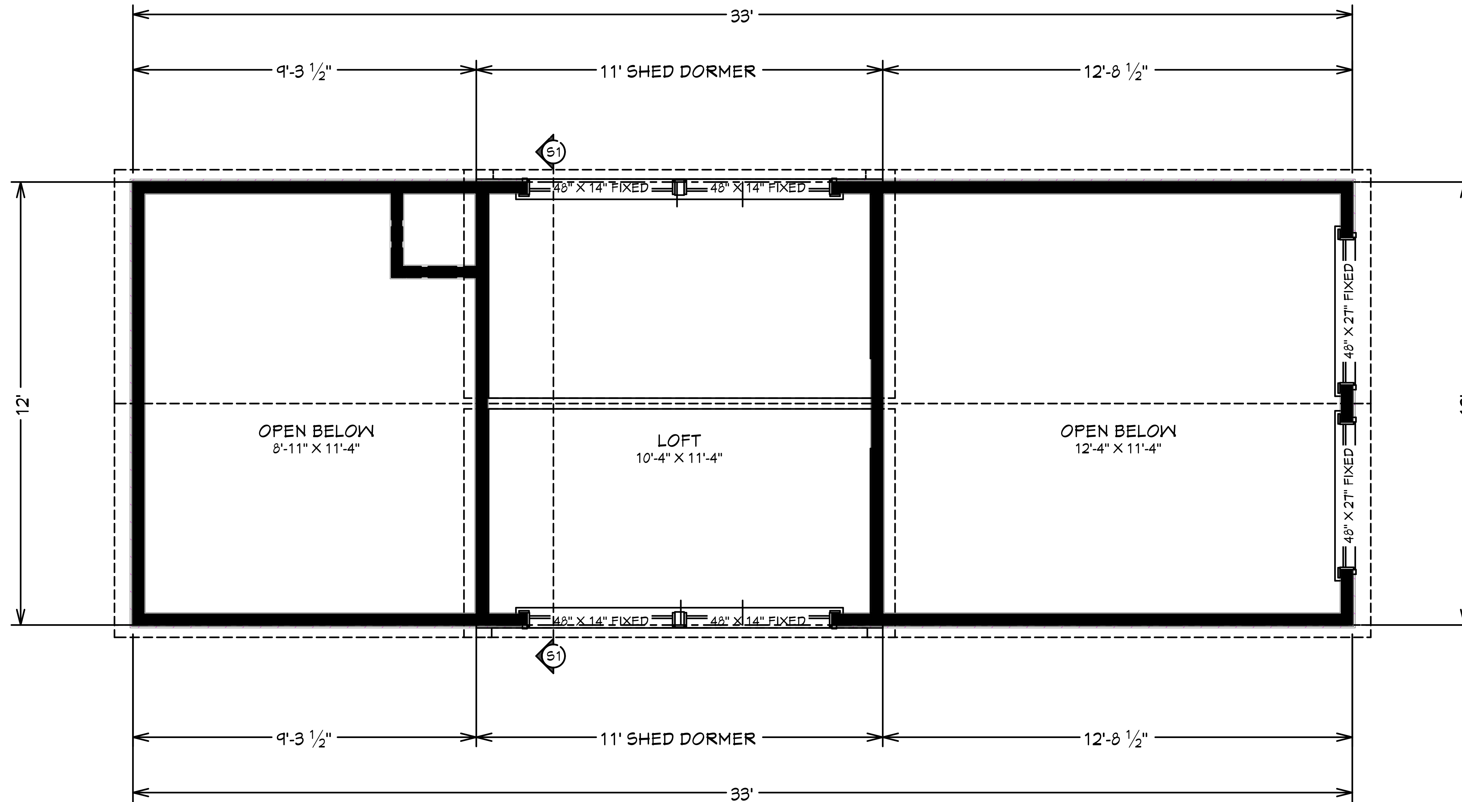
1 A-4 2ND FLOOR PLAN 5/8 IN = 1 FT
