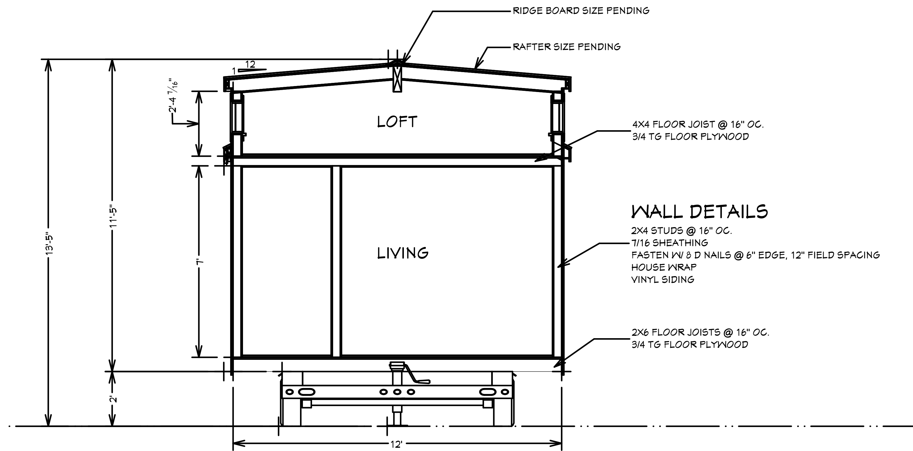
1 CROSS SECTION A-6 1/2 IN = 1 FT
