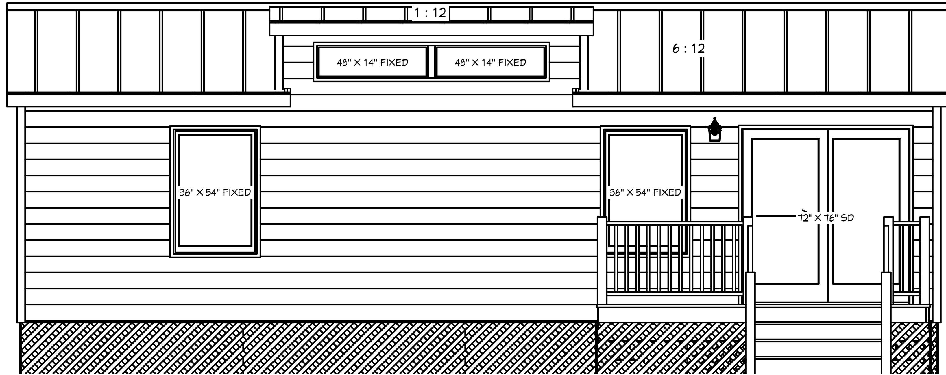
1 EXTERIOR ELEVATION FRONT A-5 1/2 IN = 1 FT
