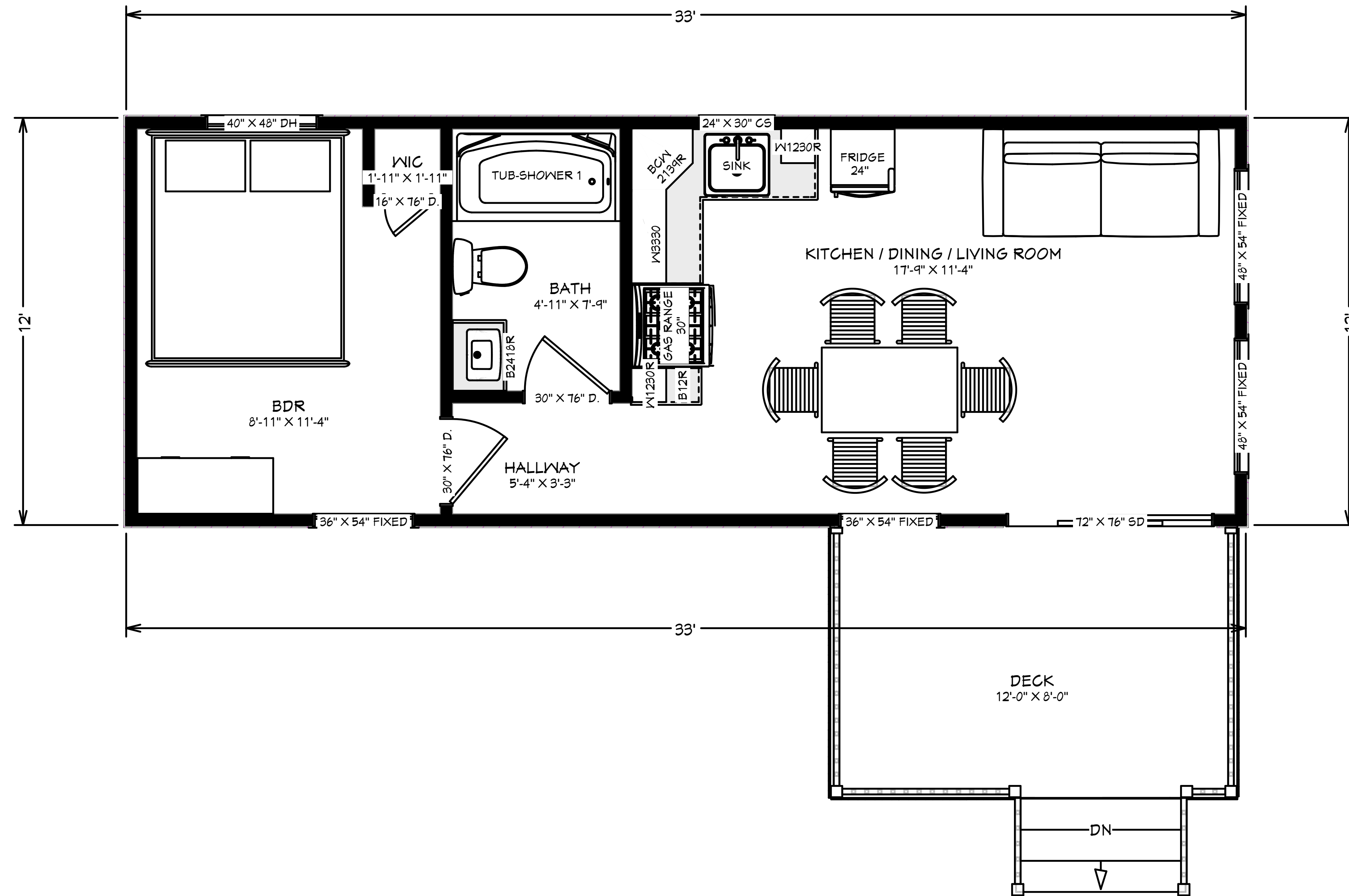
1 1ST FLOOR LAYOUT A-2 1/2 IN = 1 FT
