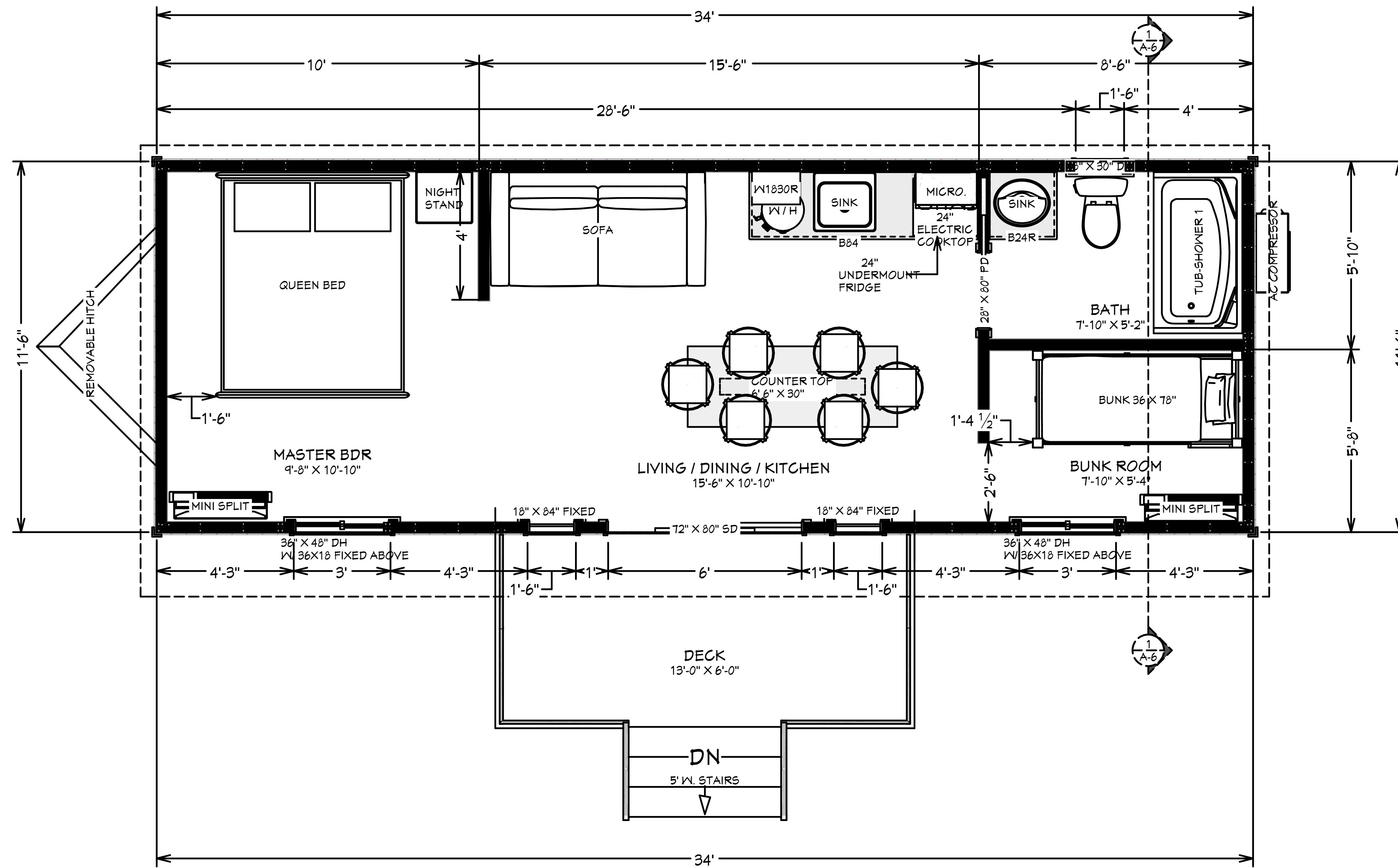
1 1ST FLOOR BUILDING PLAN A-3 1/2 IN = 1 FT
