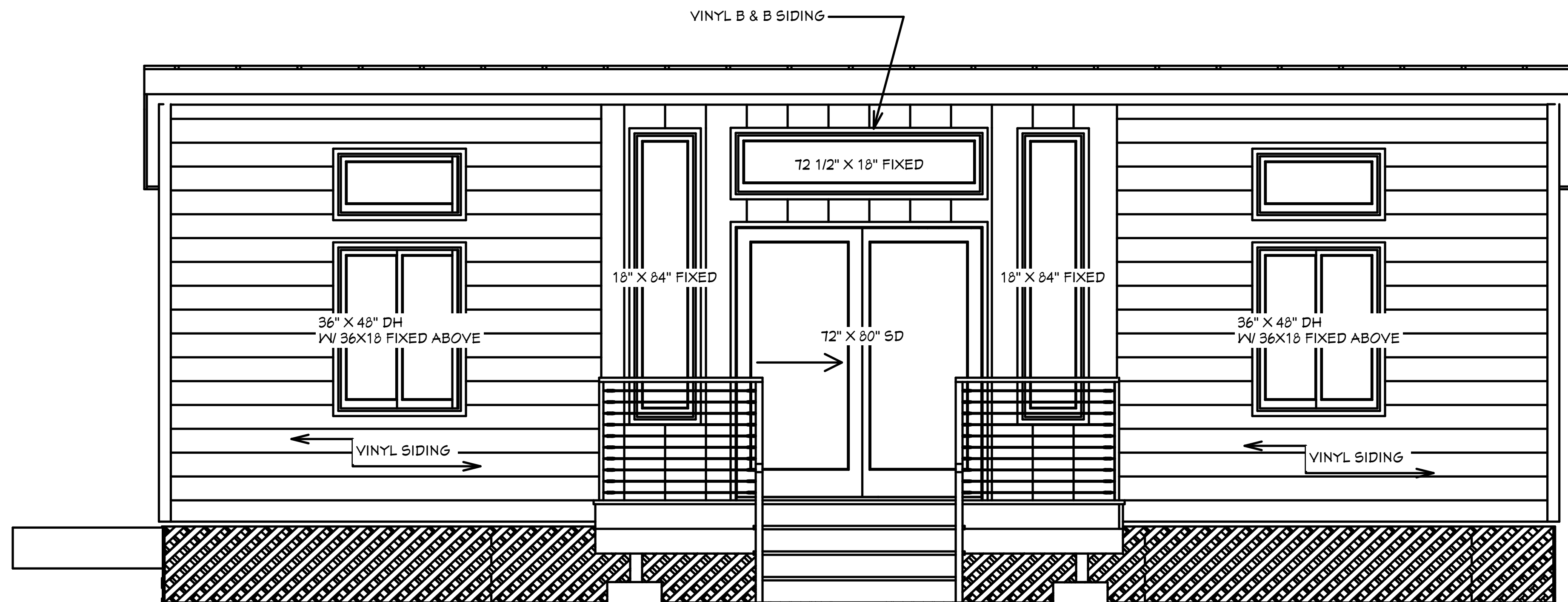
1 EXTERIOR ELEVATION FRONT A-5 1/2 IN = 1 FT
