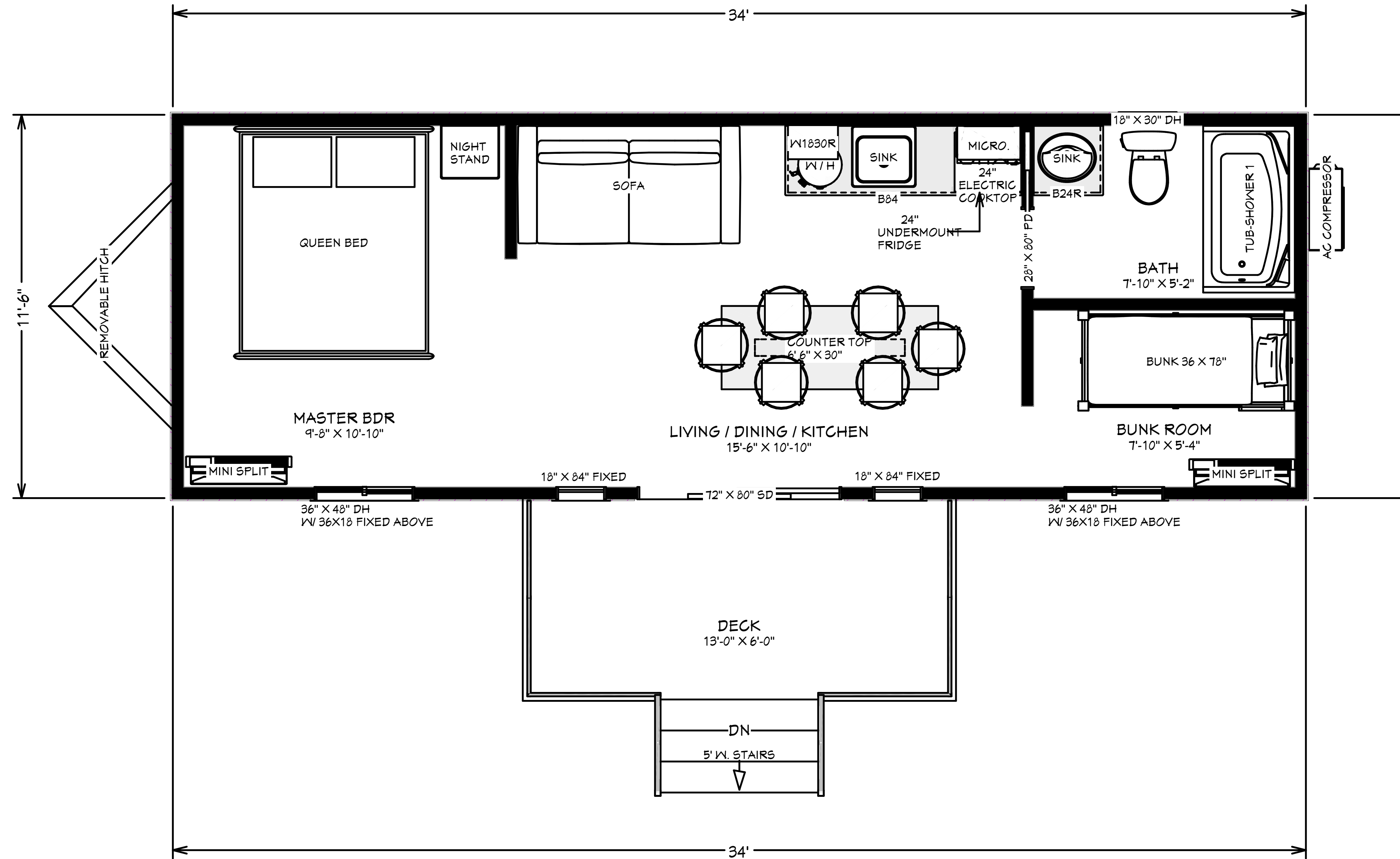
1 1ST FLOOR LAYOUT A-2 1/2 IN = 1 FT
