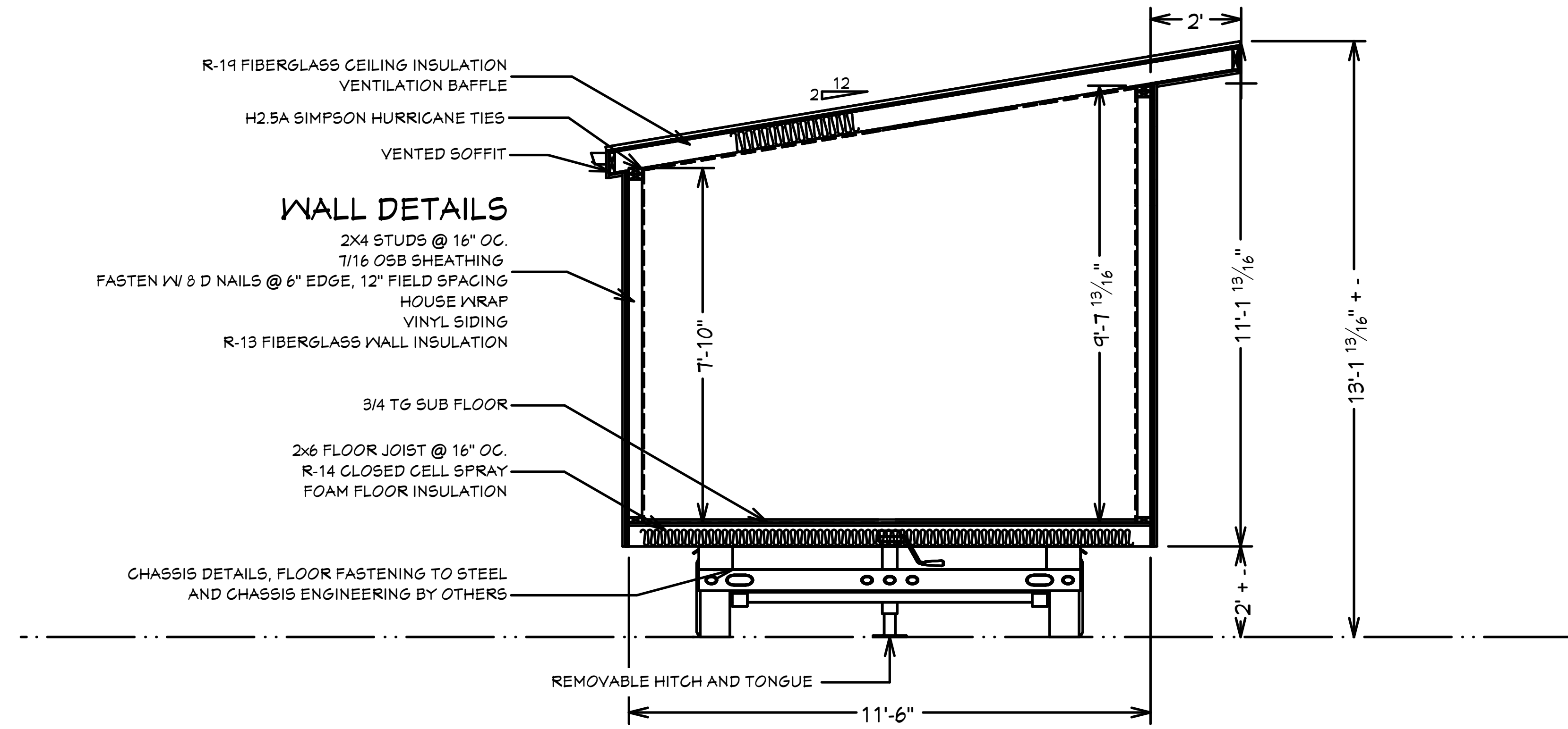
1 CROSS SECTION VIEW A-6 1/2 IN = 1 FT
