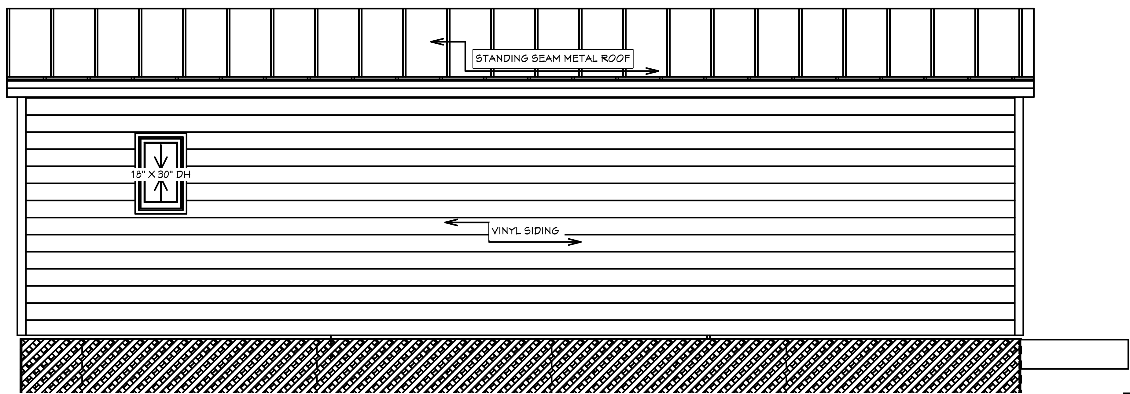
3 EXTERIOR ELEVATION BACK A-5 1/2 IN = 1 FT
