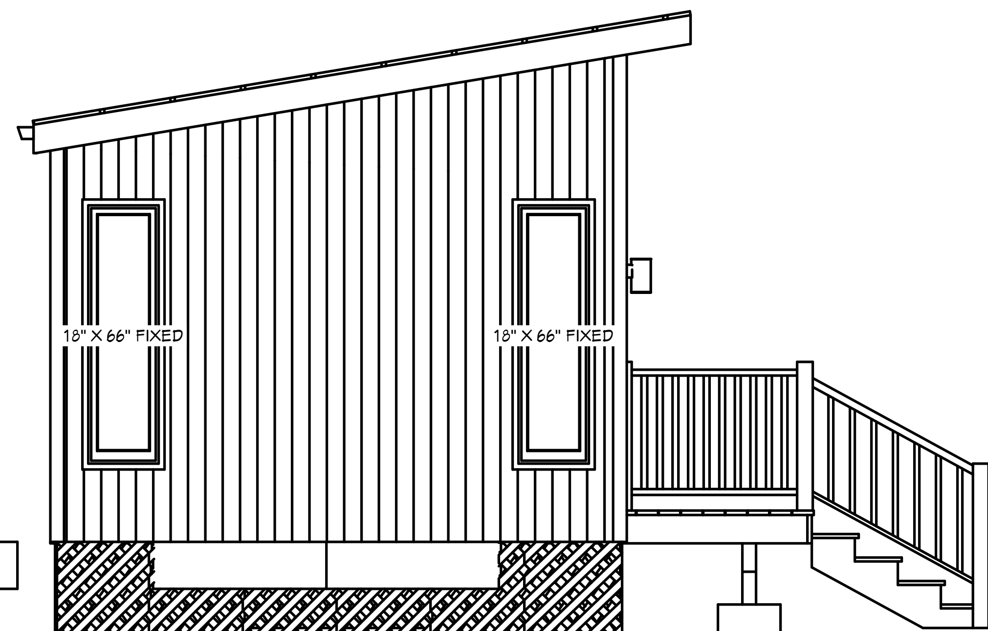
4 EXTERIOR ELEVATION LEFT A-5 1/2 IN = 1 FT
