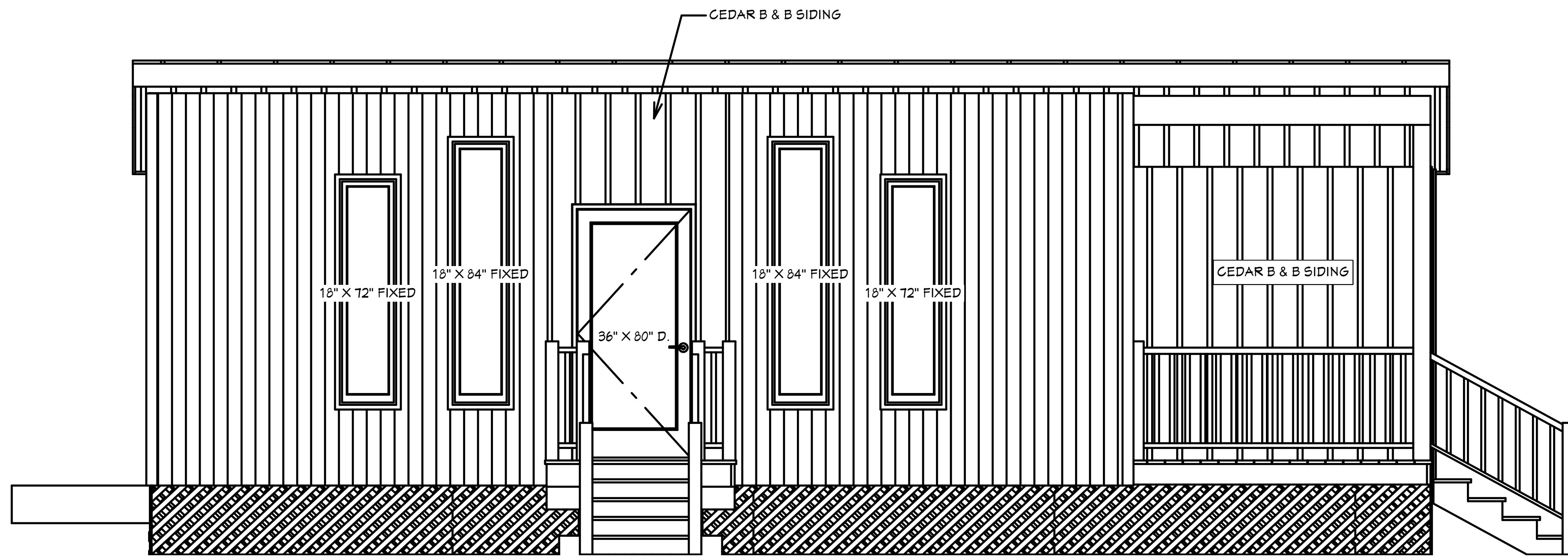
1 EXTERIOR ELEVATION FRONT A-5 1/2 IN = 1 FT
