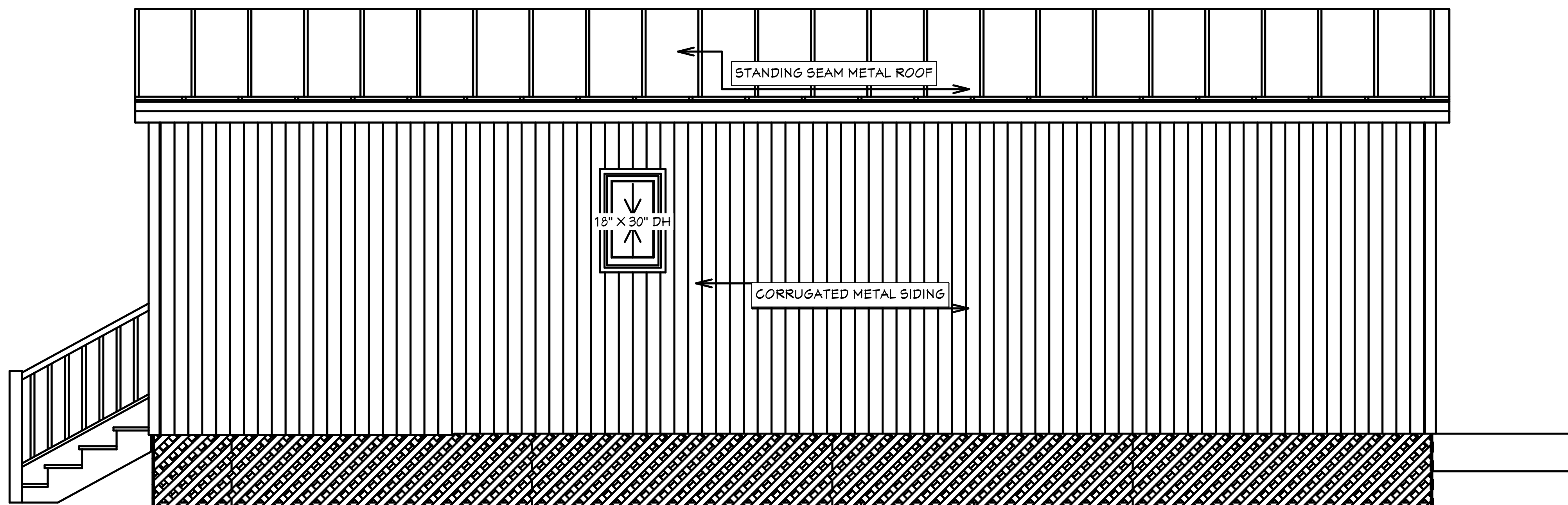
3 EXTERIOR ELEVATION BACK A-5 1/2 IN = 1 FT
