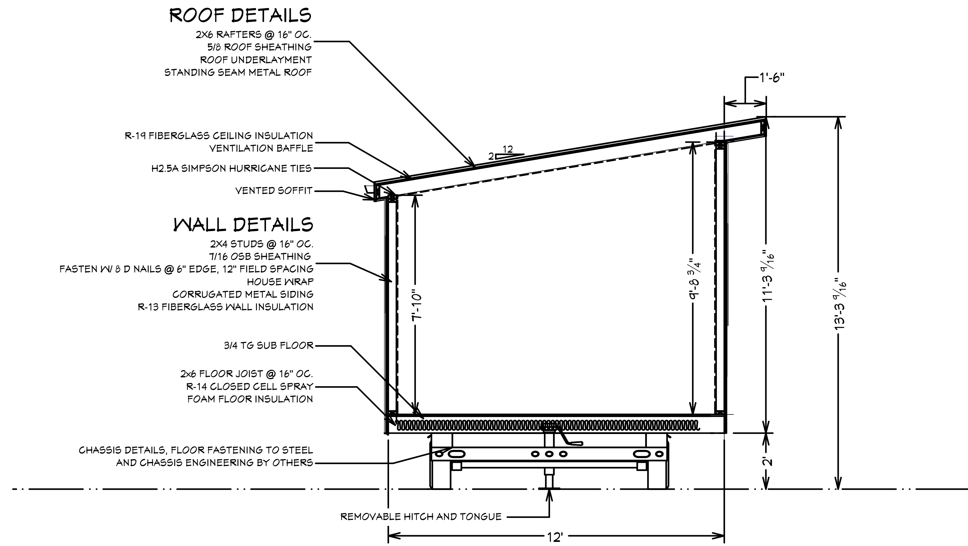
1 CROSS SECTION VIEW A-6 1/2 IN = 1 FT
