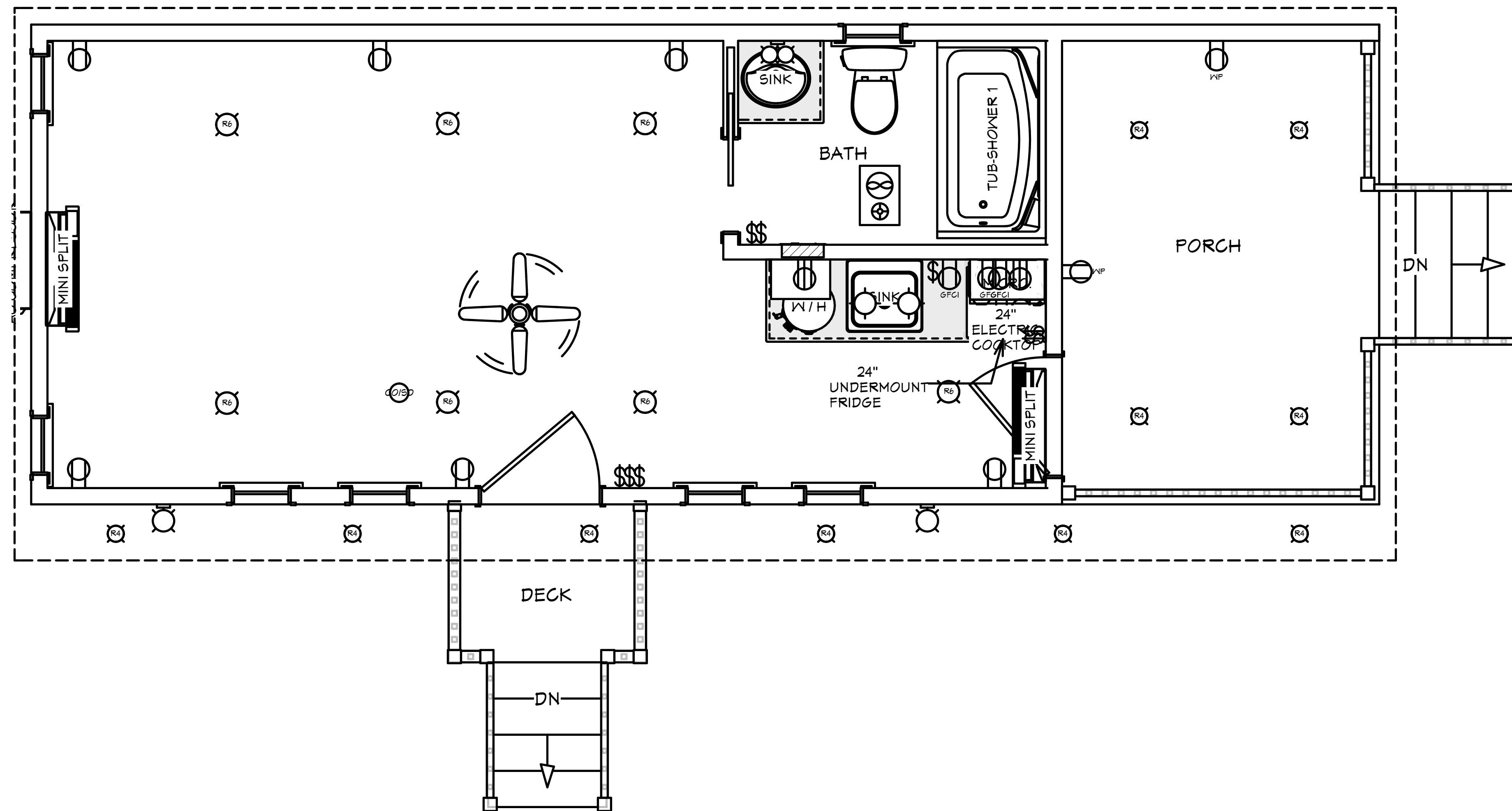
1 ELECTRICAL SCHEDULE A-4 1/4 IN = 1 FT
