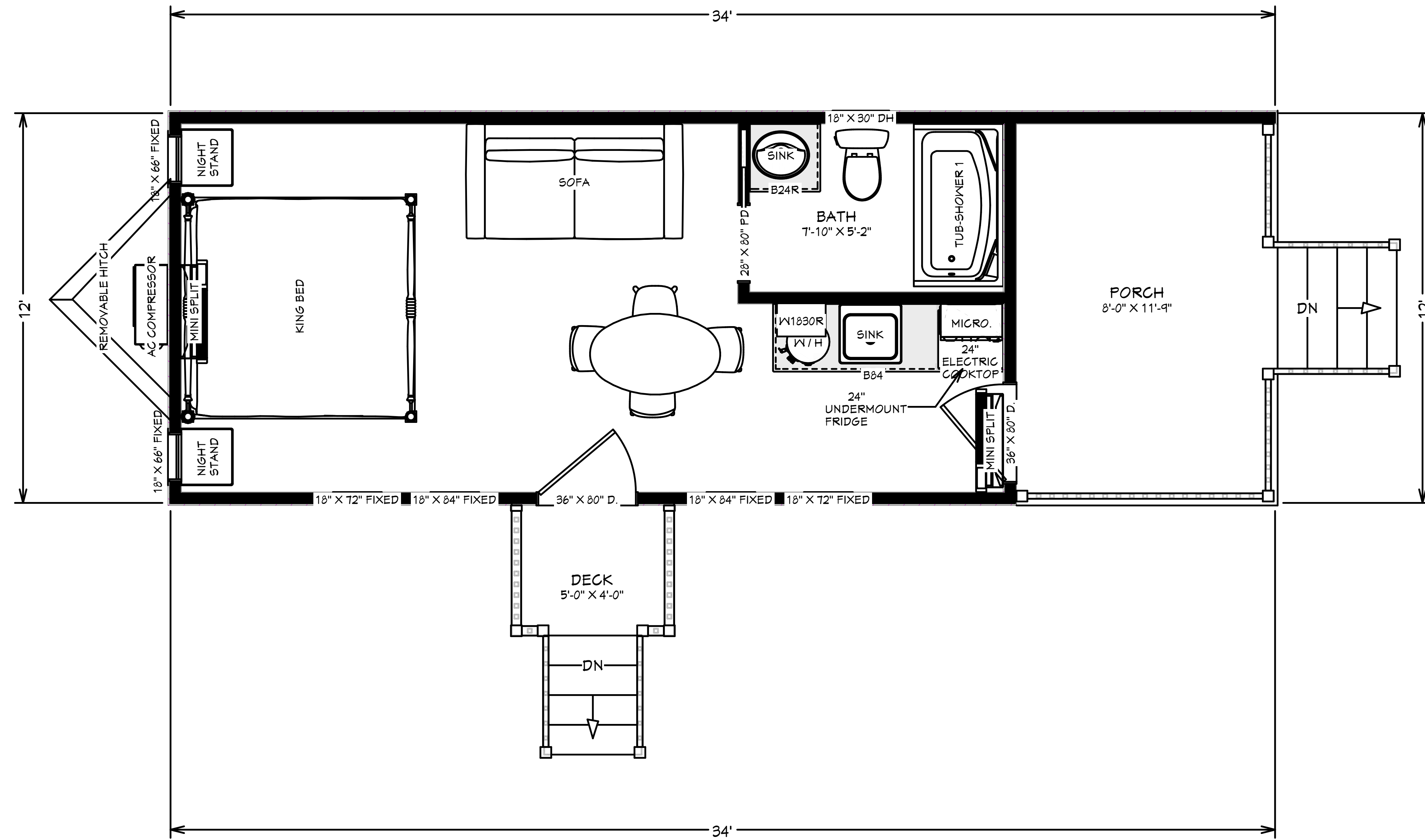
1 1ST FLOOR LAYOUT A-2 1/2 IN = 1 FT
